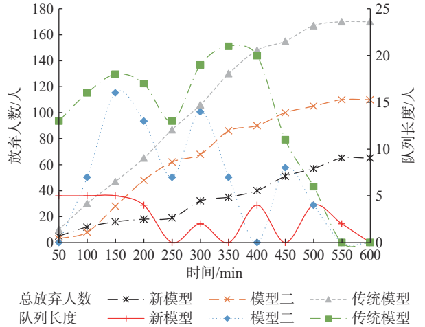
图 3 放弃人数与队列长度随时间变化的对比图 Fig. 3 Comparison of queue length and number of abandonment with time
