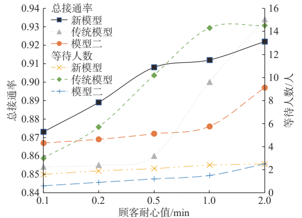
图 4 总接通率与等待人数随顾客耐心值变化的对比图 Fig. 4 Comparison of total connection rate and the waiting number of three models with customer patience value
